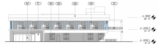
3 NORTH ELEVATION - BLDG A A301 1/16" = 1'-0"
