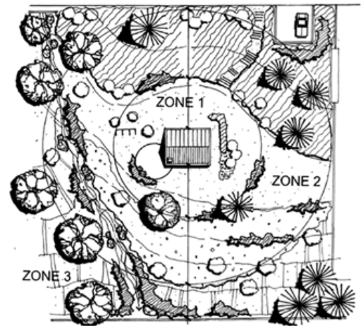
Firescaping with three zones around a house or structure to increase fire-resiliency: Zone 1 extends from the structure to 30 ft., Zone 2 is 30 to 70 ft., and Zone 3 is 70 to 120 ft. Illustration from Richard Kent's book Firescaping (Wilderness Press 2005).
